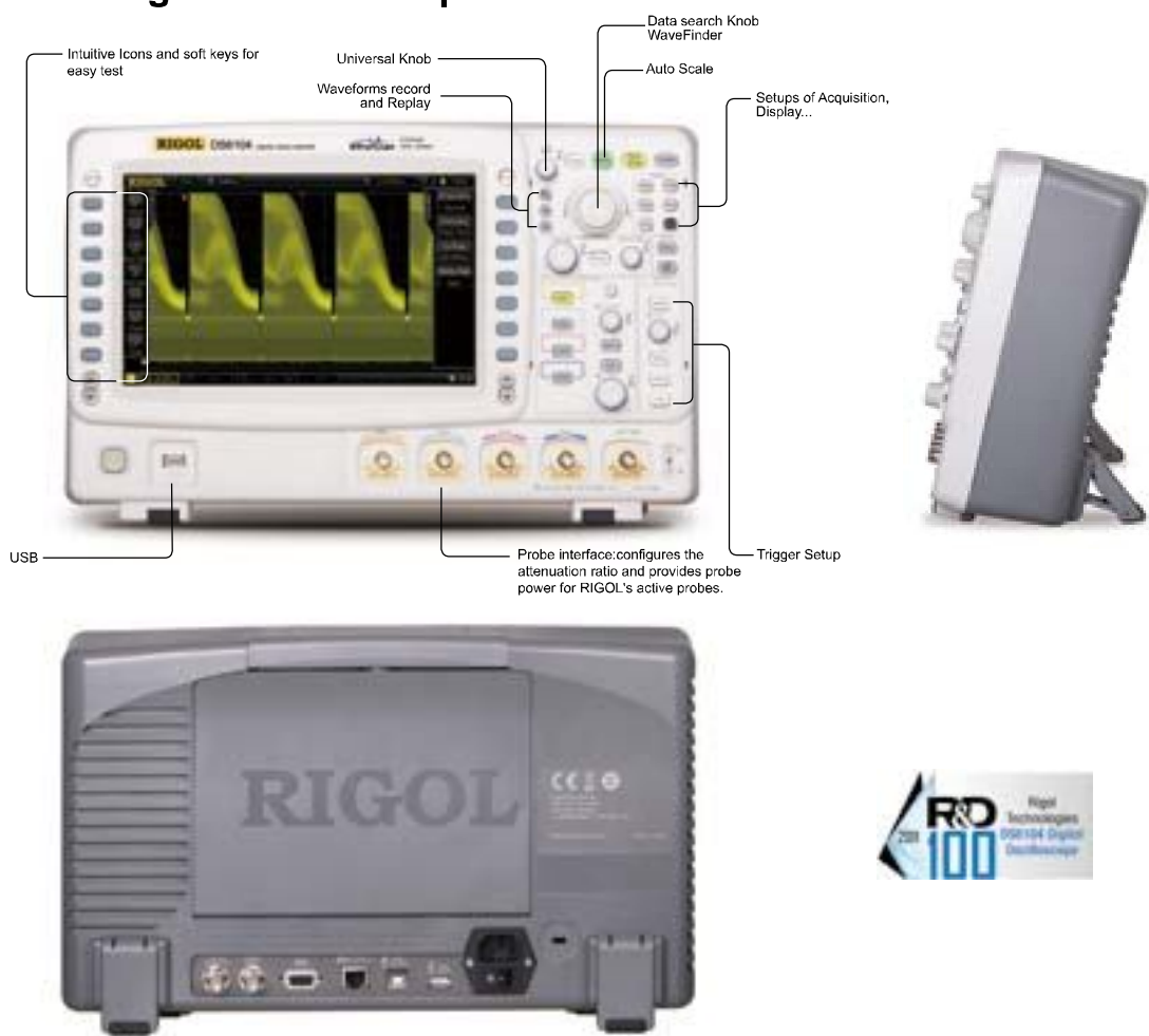
Product Dimensions: Width x Height x Depth=399mm x 255.3mm x 123.8mm Weight:5.35 kg
